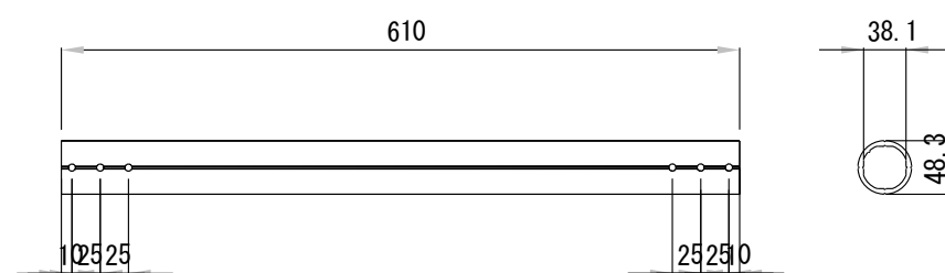
CPA-024 ( L=610mm )
