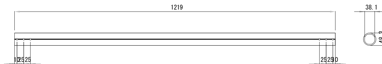
CPA-048 ( L=1219mm )
